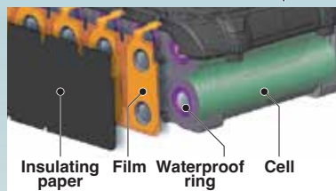
Waterproof Triple-layer Structure prevents cell failure due to water and dust
