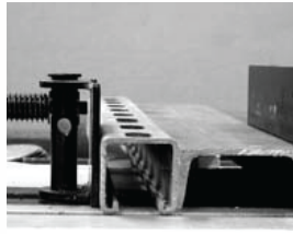
Channels & UNISTRUT™ (use block spacer)
