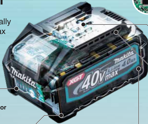
Terminal short-circuit prevention structure
